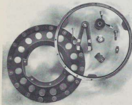
Magneto Parts
