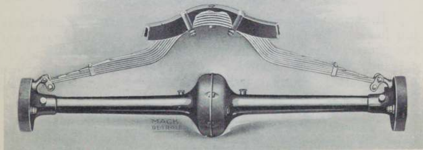
Rear Spring and Housing of Differential
